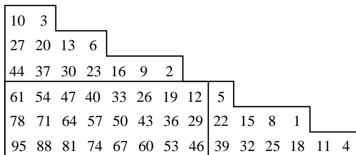
Figure 2: The (7, 17) -diagram
