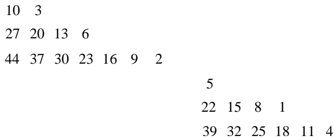
Figure 3: The (7,17) Yin and Yang diagrams
