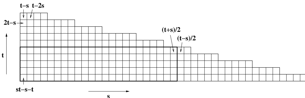
Figure 1: The (s, t) -diagram
